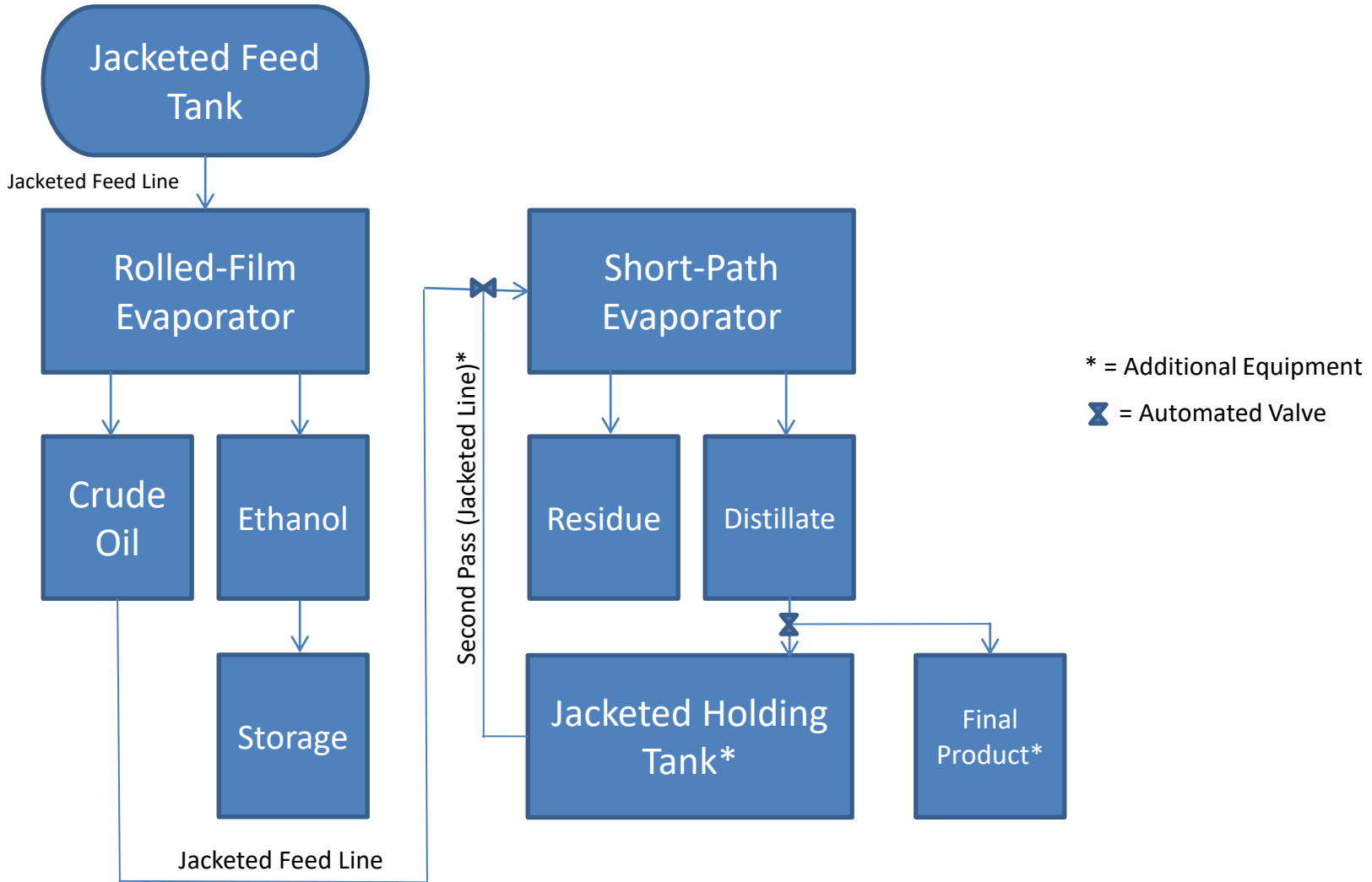
STAGE 1: ROLLED-FILM
