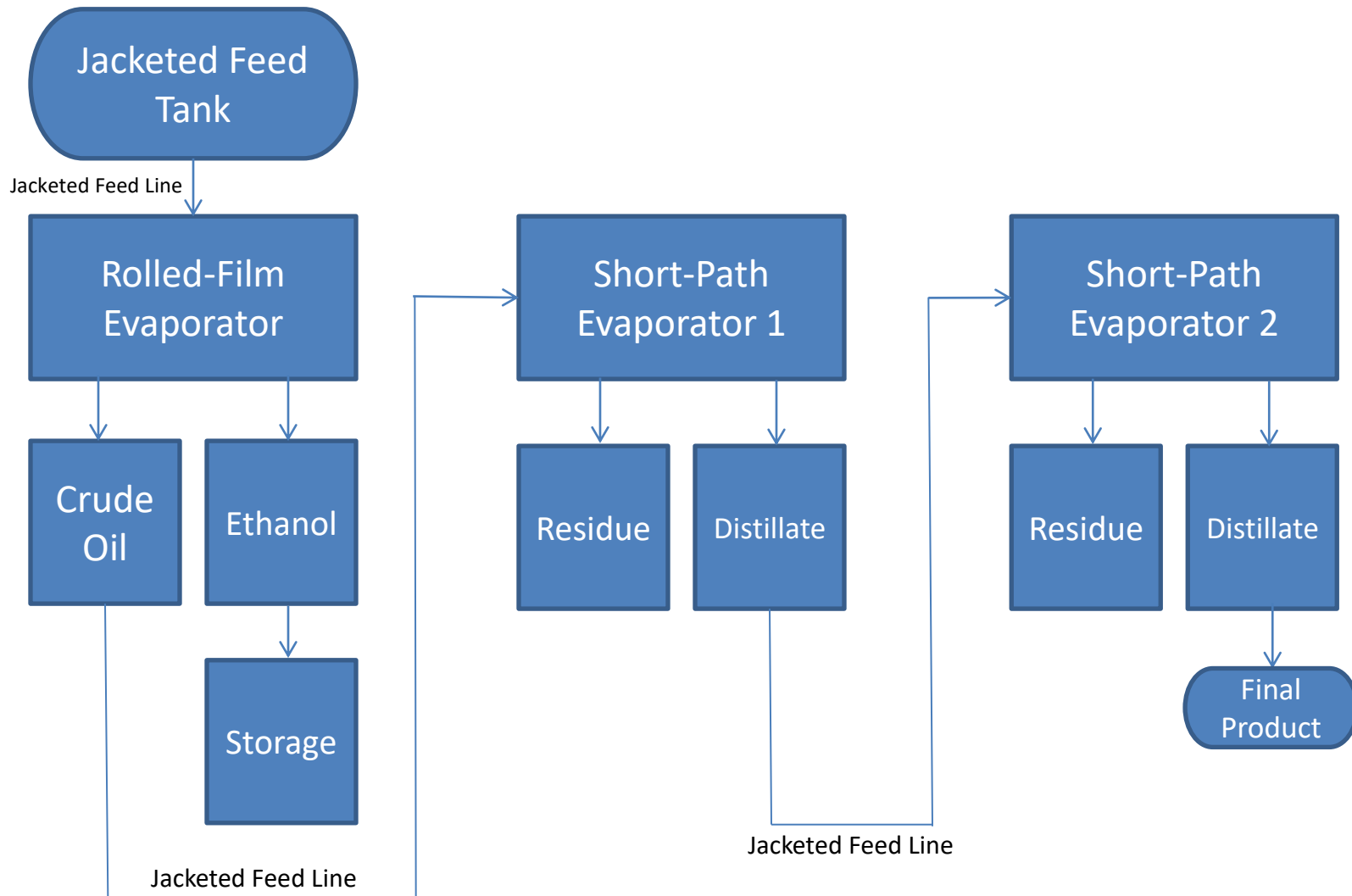
STAGE 1: ROLLED-FILM
